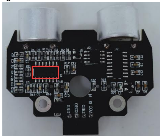
6-1 Position of chip
