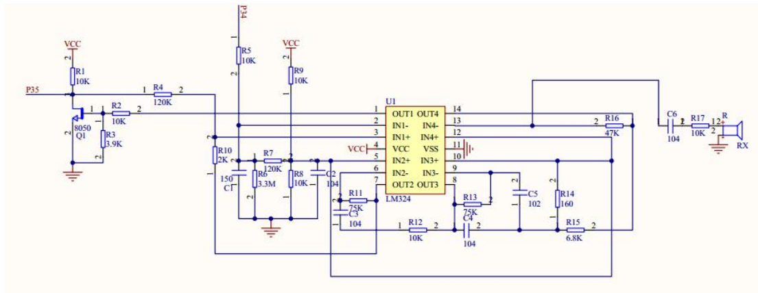
6-2 Schematic
