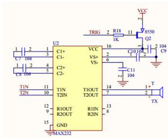
5-1 Position of chip
