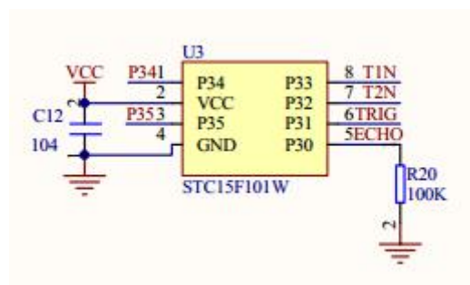
4-1 Position of MCU
