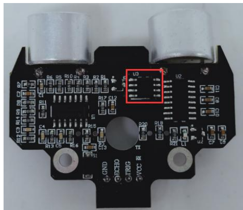
4-1 Position of MCU
